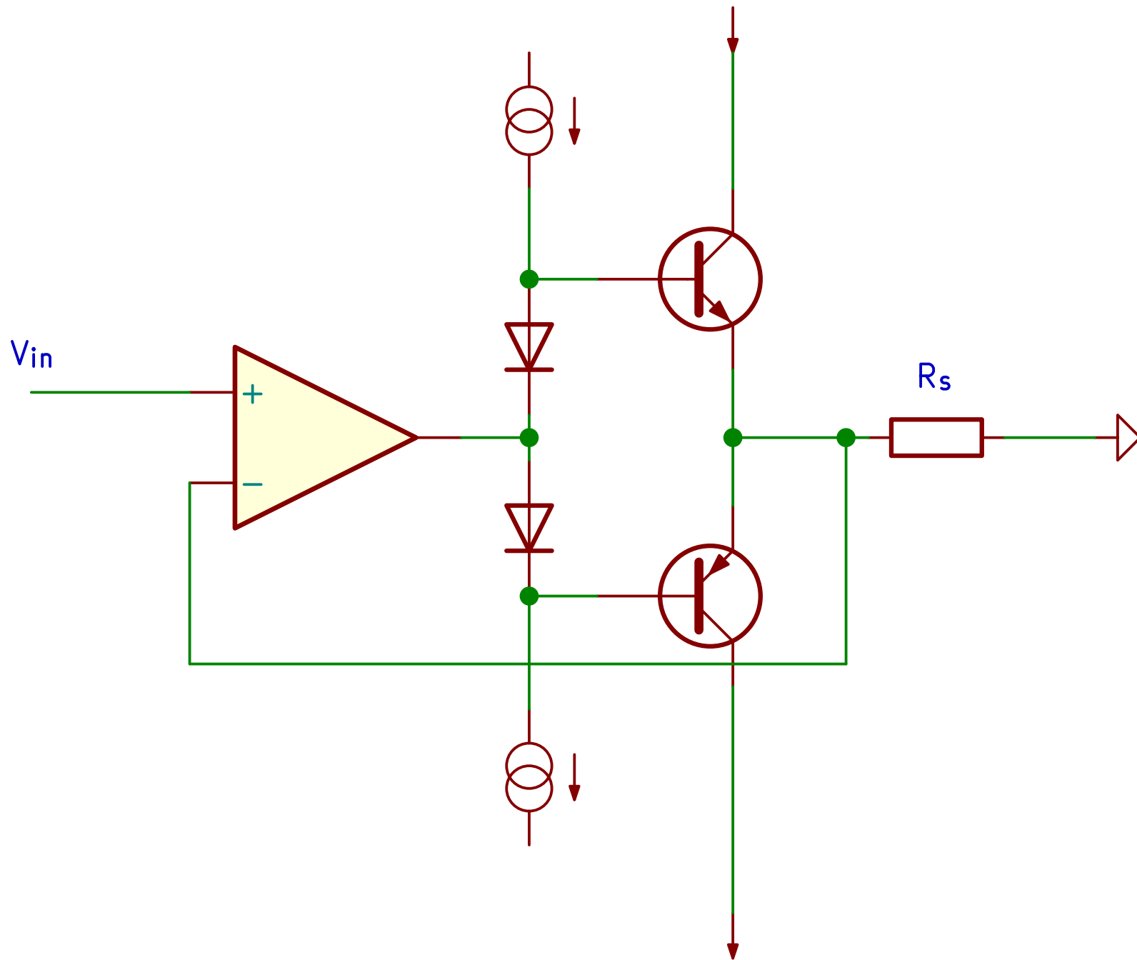
Figure 4 from 'Audio Amplifier with Defined Output Impedance' by John Howard, available at robinet.co.uk Licensed under a Creative Commons Attribution-NonCommercial-ShareAlike 4.0 International License
